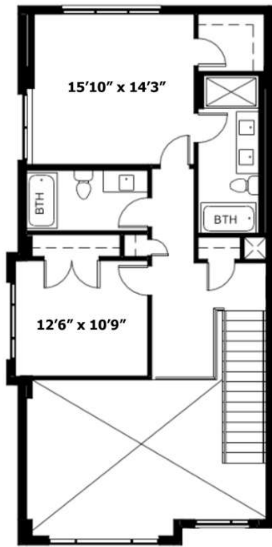
Level 2
